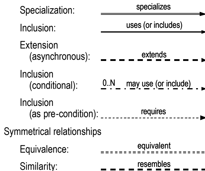
Figure 5 - Relationships in use case maps.
